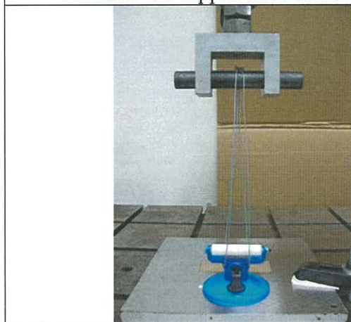
Photo "C" Horizontal tensile test
